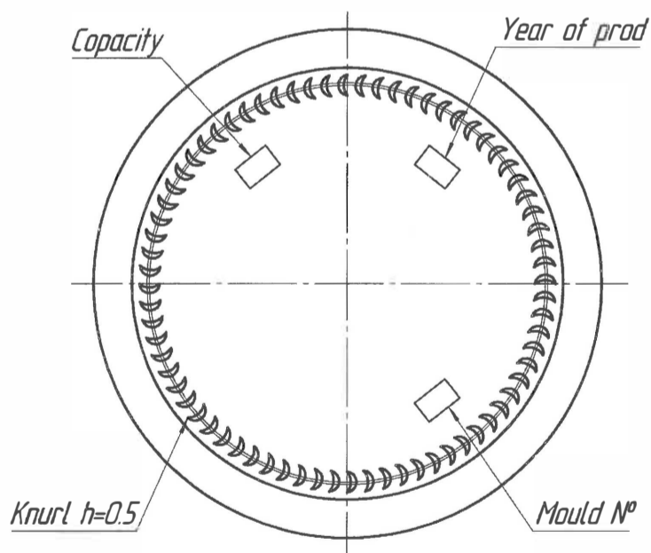
Bottom view
