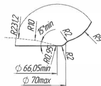
View A 2:1
